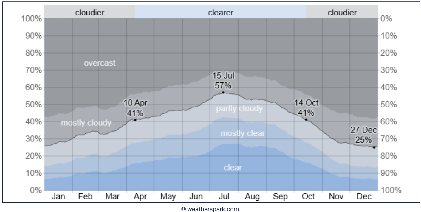
Figure 6.1: Cloud Cover at Broughton
